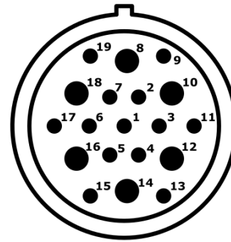
Connector from engine
